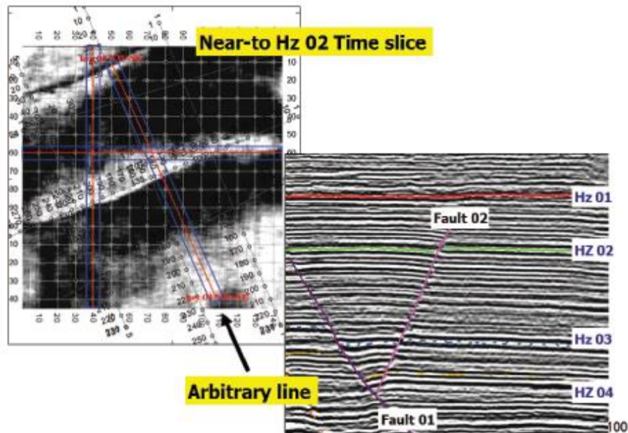
Seismic interpretation of extensional structures from a 3D survey
