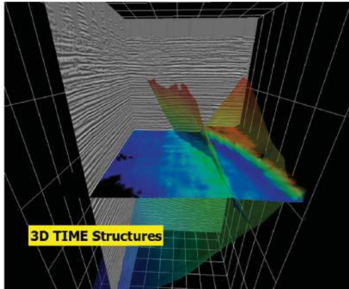
3D Structural Model building and validation
